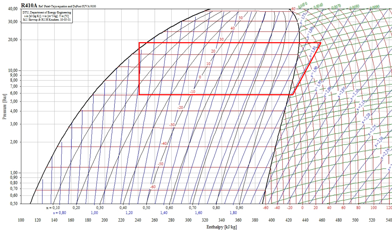
Graphical representation of inverse cycle on diagram p-h
